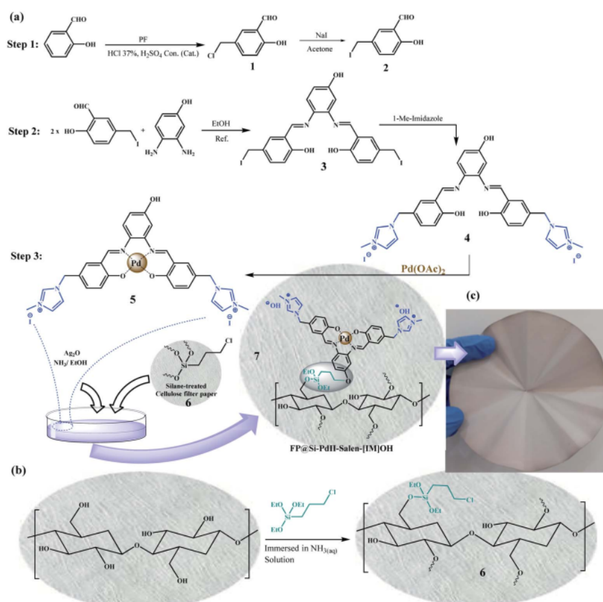
34 Scheme 1 The synthesis of (a) \text{Pd}(\text{II}) -salen-[IM] complex (5) and \text{FP@Si-Pd}^{\text{II}}\text{-Salen-[IM]OH} (7), and (b) silylation of the cellulose filter paper by CPTES ( \text{FP@Si-Cl} ). (c) Original picture of the prepared \text{FP@Si-Pd}^{\text{II}}\text{-Salen-[IM]OH} filter paper.
